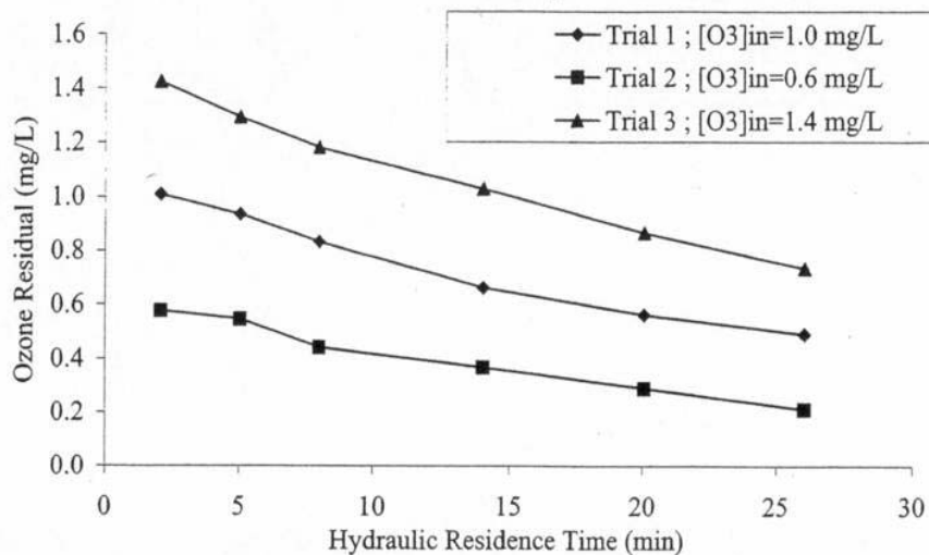
Figure 4 Ozone decay profiles at pilot-scale at Chertsey WTP (UK) [O3] in : ozone residual at the inlet of the contactor (or outlet of the gas-liquid separator) Chandrakanth, 2001
